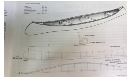
Construction of a wooden canoe
